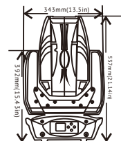
200W 3in1 Spot Beam Wash Moving Head FO-LM200C
