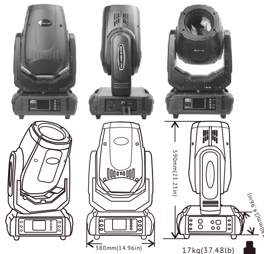
350W 3in1 Spot Beam Wash Moving Head
